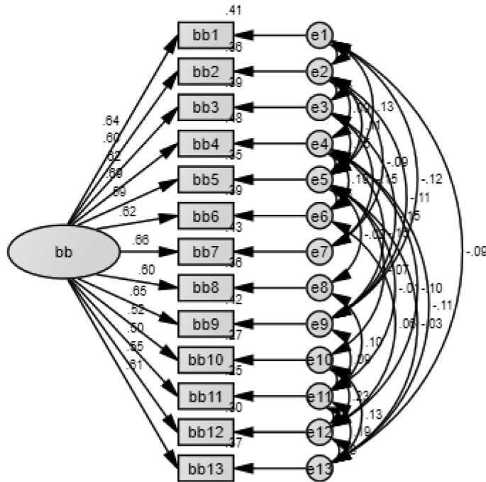
Model_bb
