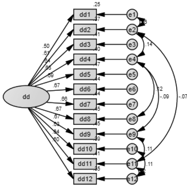
Model_dd
